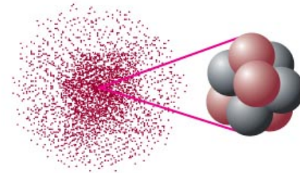
Carbon ( {}^{12}\text{C} )
