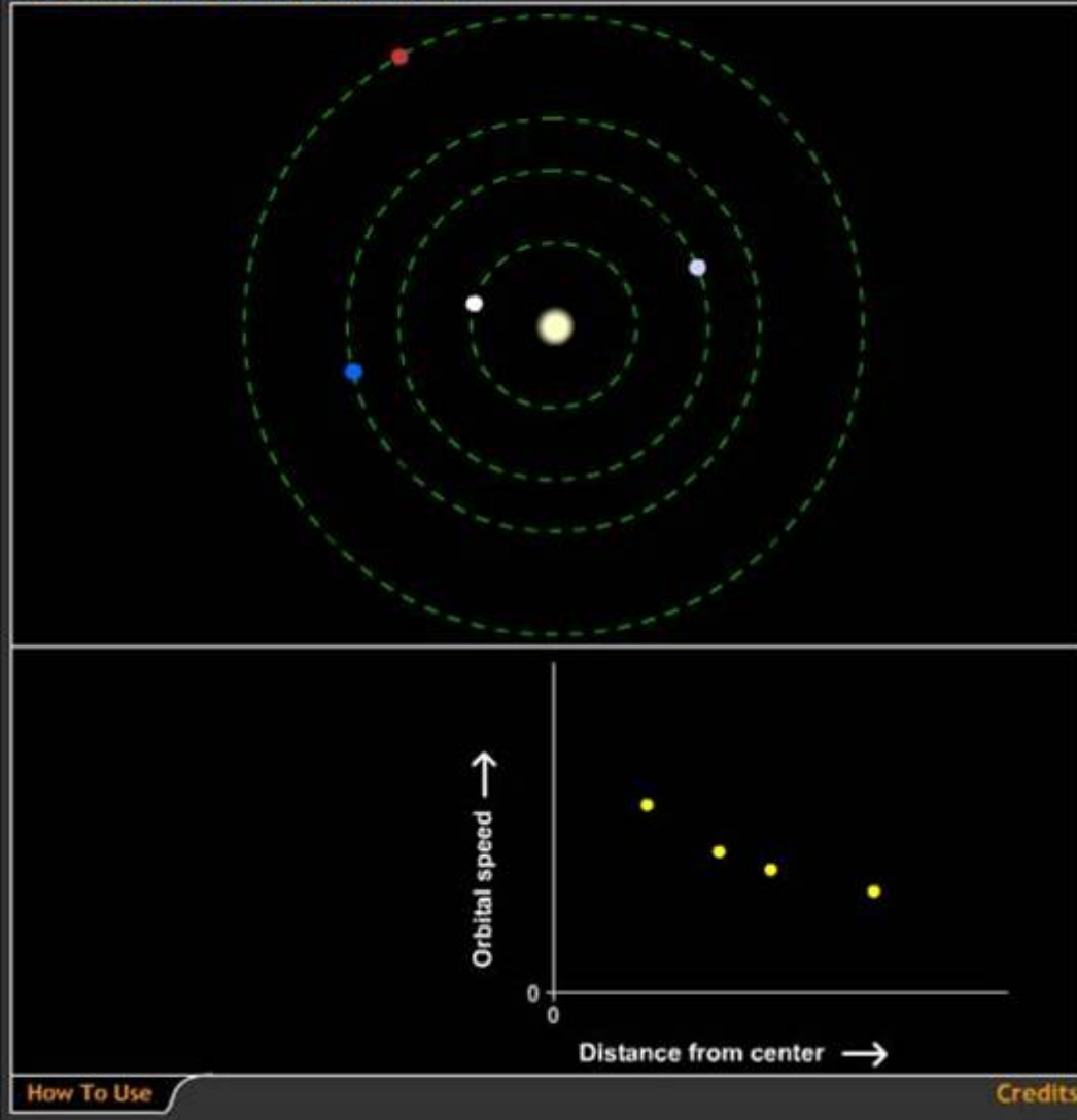
Rotation Curve of the Solar System
