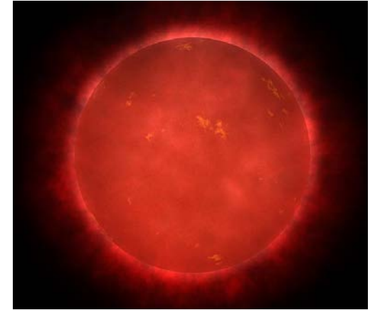
Artistic presentation of a red dwarf star.
